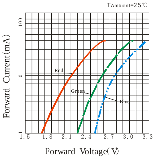
Volt-Ampere Characteristics
