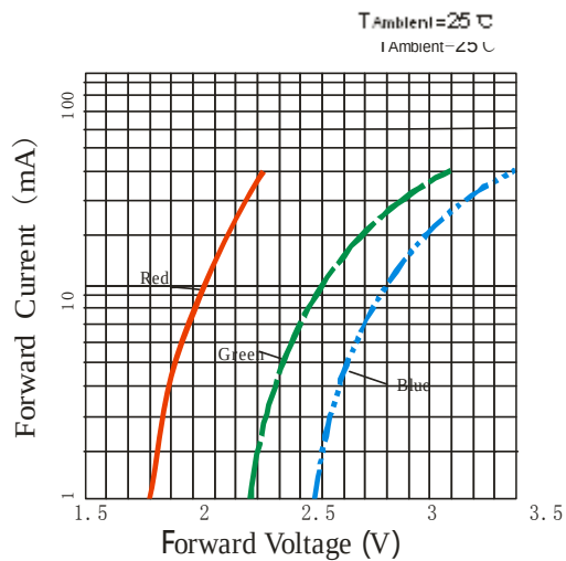
Volt-Ampere Characteristics
